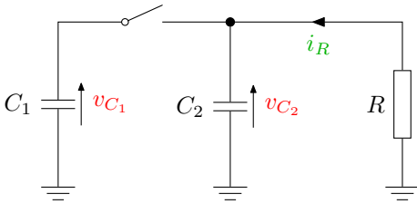
Fig. 2: A simple switching electrical circuit
