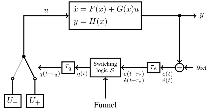
Fig. 2: Overall system structure with time delays in the error signal and the input.
