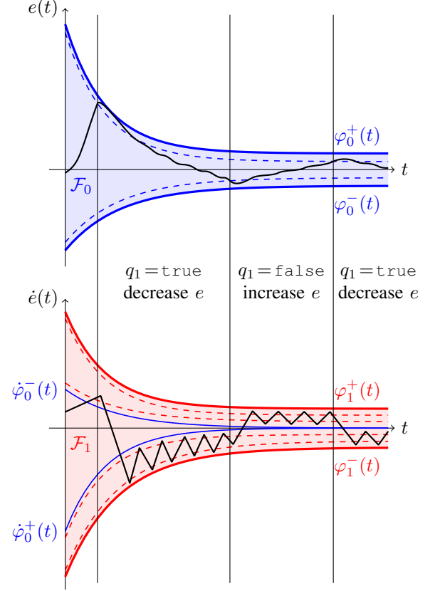
Fig. 1: A schematic illustration how the error (upper part) and its derivative (lower part) evolve in closed loop with the bang-bang funnel controller in the presence of time delays. The dashed lines denote the safety distances.
